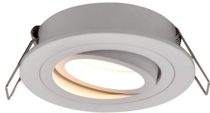
3. CHUCK DL ROUND | Spot ARGU10-038-N 1 x GU10 MAX 50W aluminium white body
